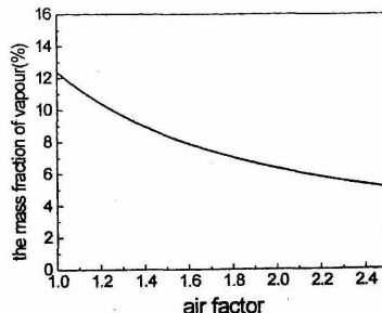
Fig.2 mass composition of humidity in flue gas as a function of the air factor
