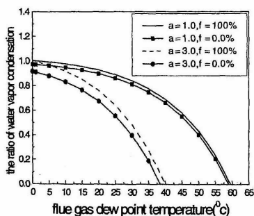
Fig.3 the curves of condensation ratios function of flue gas temperature
