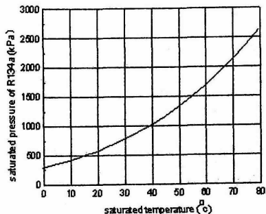
Fig.6 variation of saturated pressure with saturated temperature for R134a
