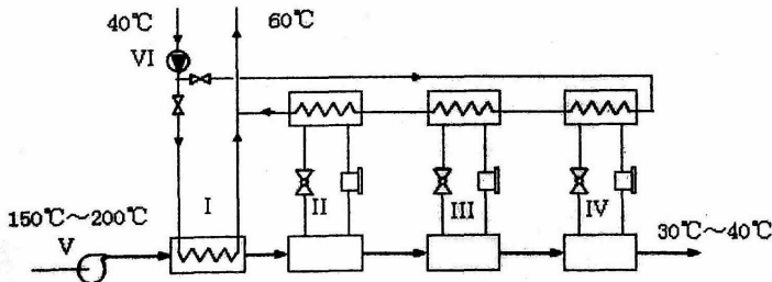
Fig.5 flue gas heat pump technical flow chat
