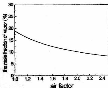
Fig.1 volume composition of humidity in flue gas as a function of the air factor
