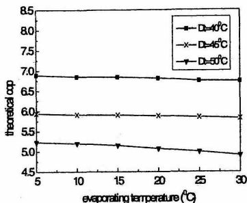
Fig.7 theoretical COP against the evaporating temperature for R134a
