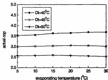
Fig.9 actual COP against evaporation temperature
