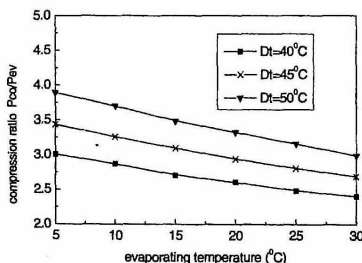
Fig.8 compression ratio against evaporation temperature
