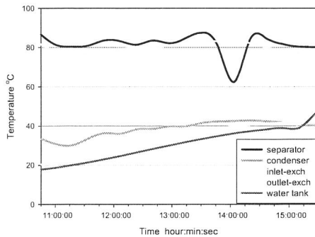
Graph 1: Temperature of the system
