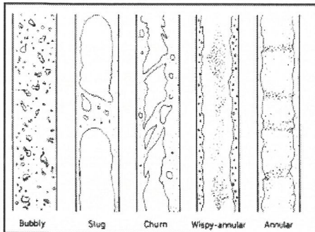
Figure 2: Flow patterns in the vertical co-current flow
