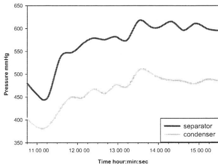
Graph 2: Pressure of bubble pump
