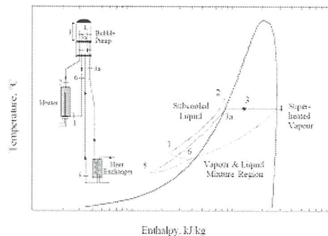
Figure 5: Thermodynamic cycle of bubble pump
