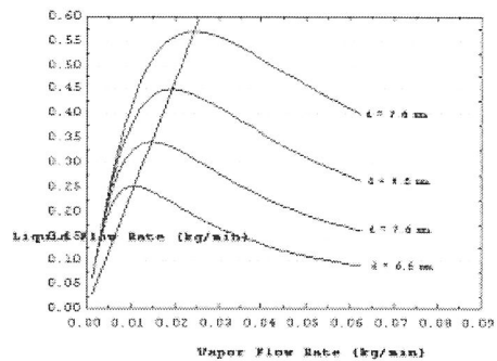
Figure 3: Bubble pump performance for varying tube diameter and a fixed h/L=0.2
