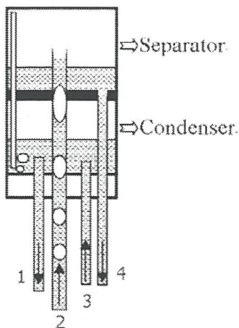
Figure 4: the structure of bubble pump
