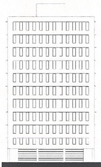
Figure 4: Main façade for building Pedro de Valdivia. Santiago. Chile.
