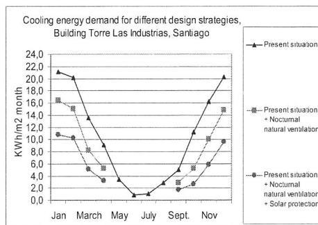
Figure 3: Cooling energy demand for building Las Industrias. Santiago. Chile.
