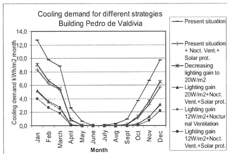
Figure 6: Cooling energy demand for building Pedro de Valdivia. Santiago. Chile.
