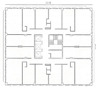
Figure 5: Plan of building Pedro de Valdivia.
