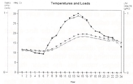
Figure 7: North façade proposal on day 200
