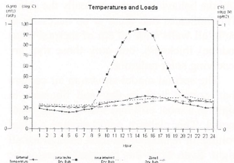
Figure 8: South façade proposal on day 59
