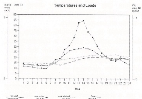
Figure 9: South façade proposal on day 200
