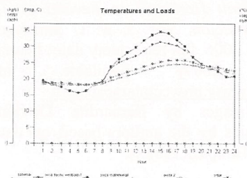
Figure 6: North façade proposal
