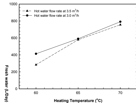
Figure 8: Fresh water generation rate with temperature and different flow rate.
