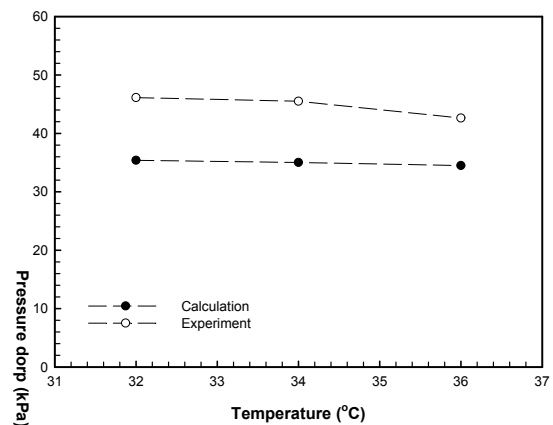
Figure 4: Comparison of pressure drop between experiment and calculation of cold water side.
