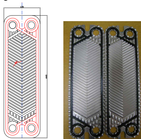
Figure 2: Plate used in the experiment.
