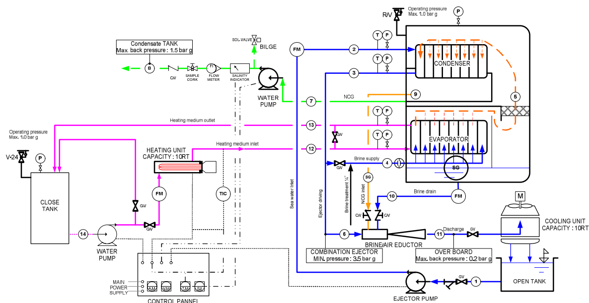
Figure 9: Diagram of the experimental facility of fresh water generator system.
