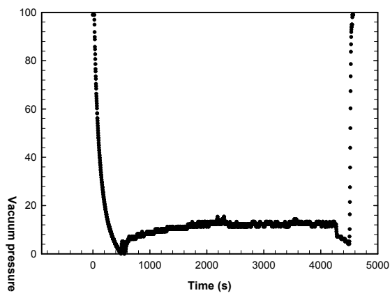
Figure 5: Vacuum pressure distribution inside of the vessel.
