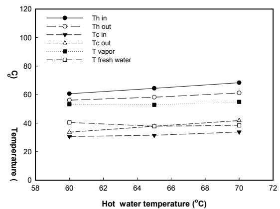
Figure 7: Mean temperature distributions with hot water flow rate of 3.5m 3 /h.
