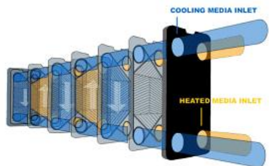
Figure 1: Flow arrangement in the plate heat exchanger with U type configuration.
