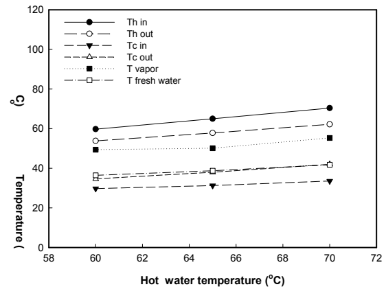
Figure 6: Mean temperature distributions with hot water flow rate of 3.0m 3 /h.
