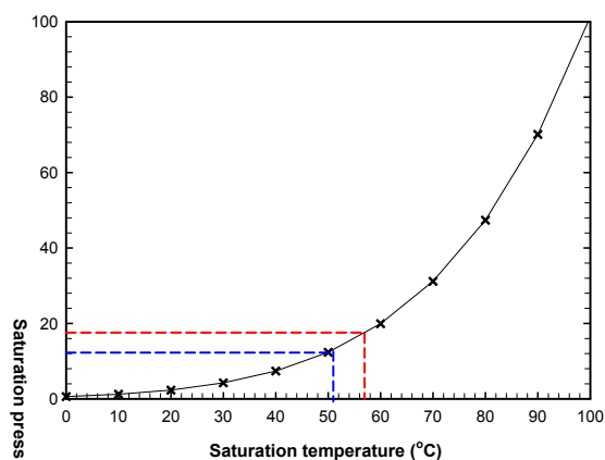
Figure 3: Saturation temperature and pressure.
